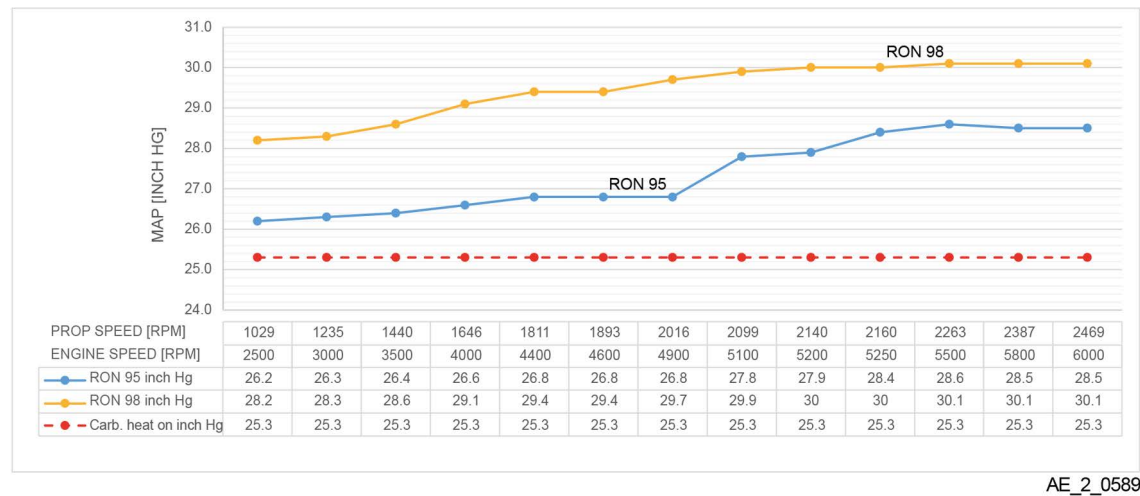
Fig. 1 Manifold absolute pressure (MAP) and engine speed settings for ROTAX® 912 S/ULS for fuel type RON 95 and RON 98*
