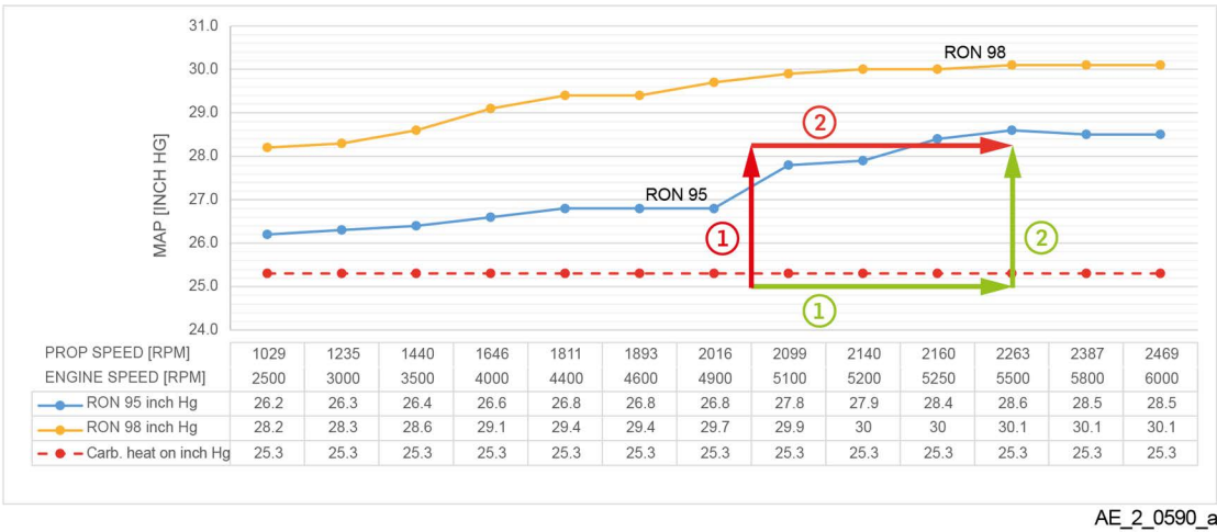
Fig. 2 Power increase
