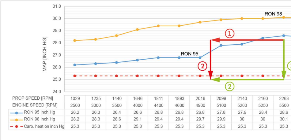
Fig. 3 Power reduction
